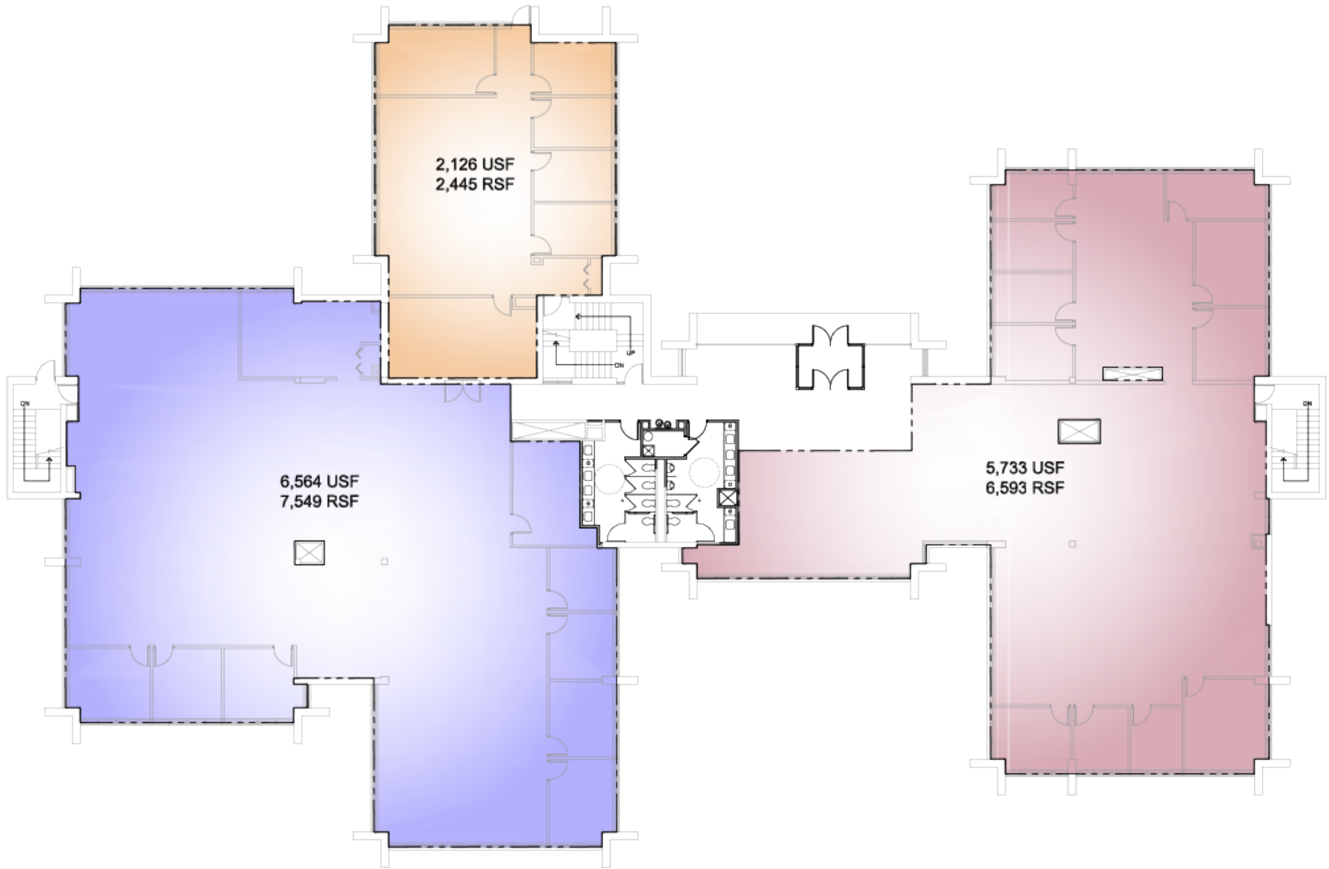
1 SECOND FLOOR PLAN SCALE: 1/16"=1'-0"
